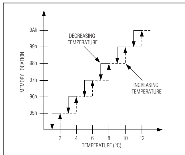
Figure 14. LUT Hysteresis
